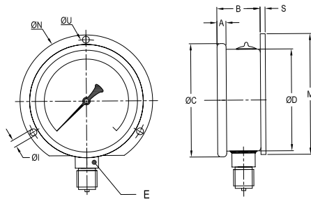
Rolling Type
